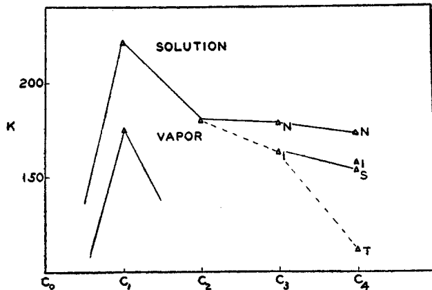
FIG. 2. Extinction coefficient (moles per liter) of the 0-0 bonds of monoalkyl-substituted benzenes.
