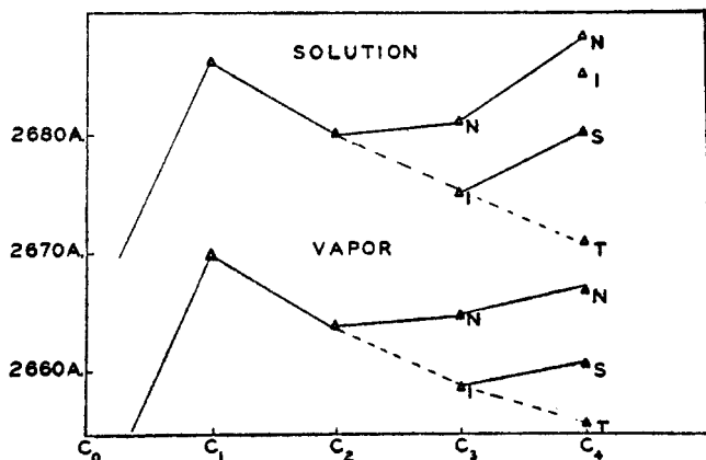
FIG. 1. Wave lengths of the 0-0 bonds in monoalkyl-substituted benzenes
